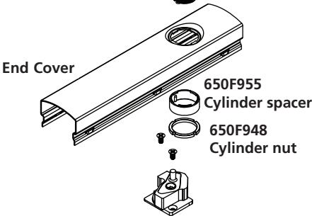
CR1000-118-A02 Cylinder
